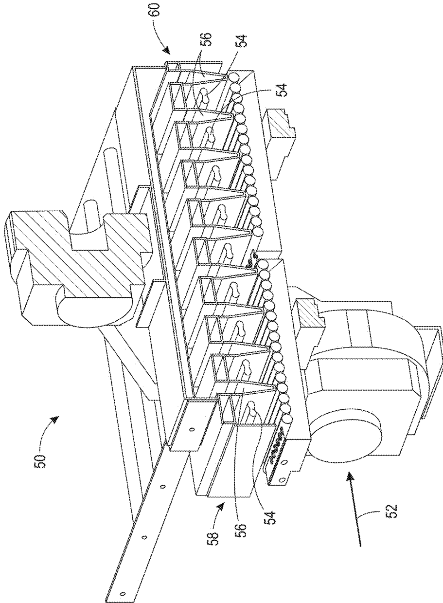
FIG. 2 PRIOR ART
