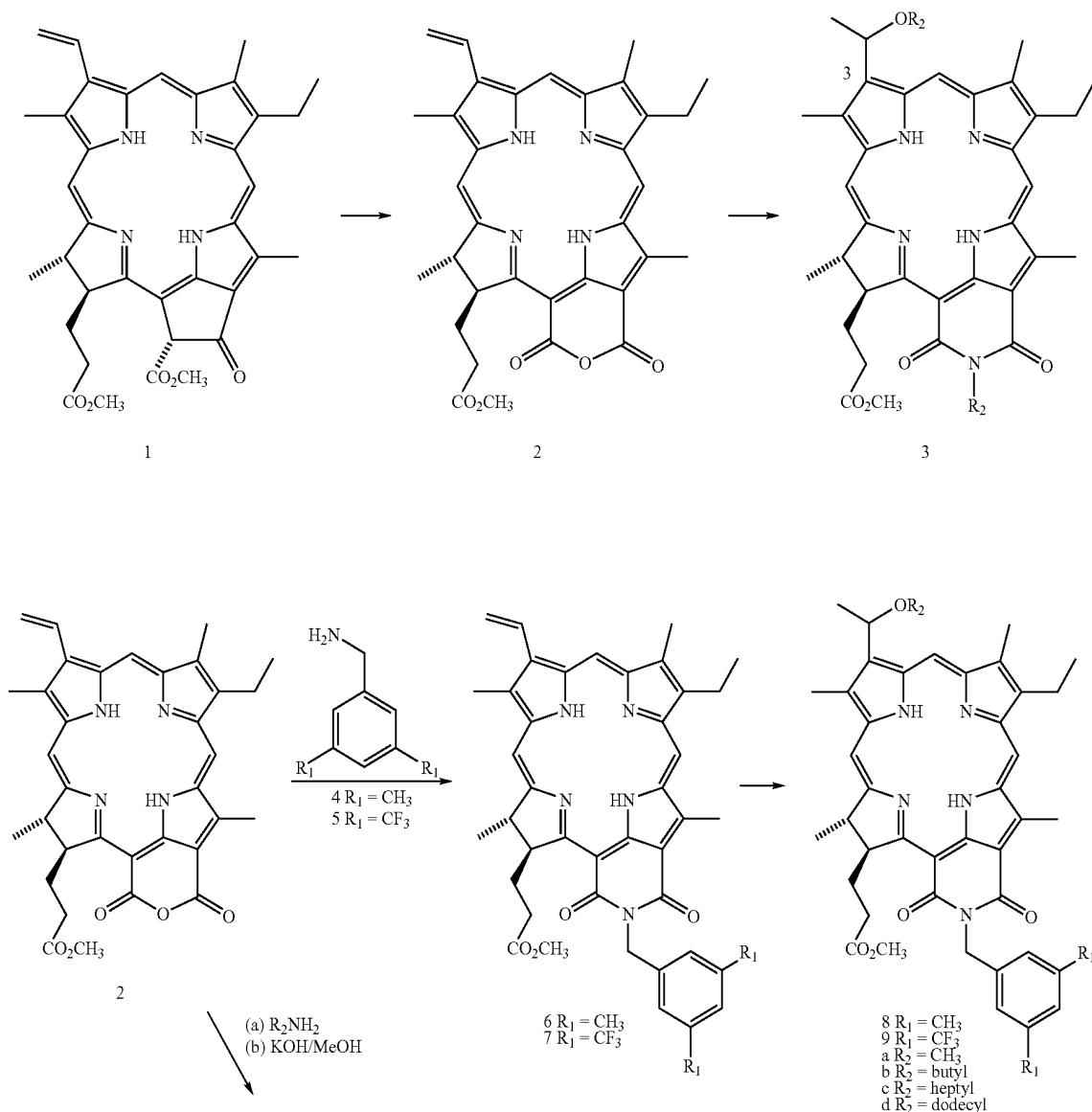
Scheme 1
