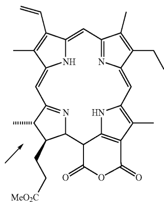
Chlorin(purpurin)
