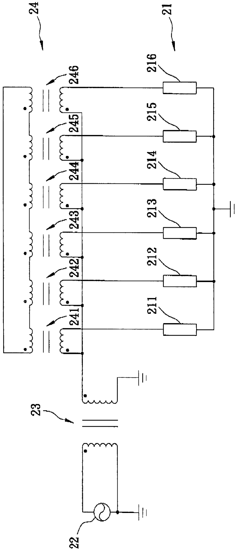
FIG. 2 PRIOR ART
